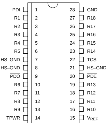
DS2109, DS2109S 28-PIN SOIC (300 MIL)
