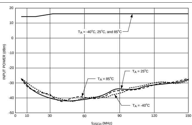
V_{CC} = 3.0\text{ V} , \text{OSC\_2X} = 0 Figure 7. OSCin Sensitivity
