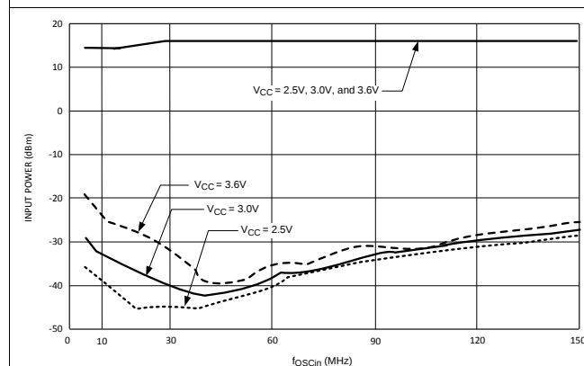
T_A = 25^\circ\text{C} , \text{OSC\_2X} = 0 Figure 6. OSCin Sensitivity
