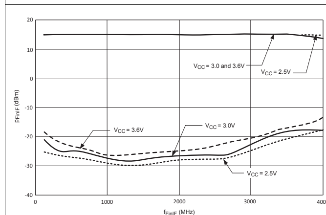
T_A = 25^\circ\text{C} , \text{IF\_P} = 16 Figure 4. IF PLL Fin Sensitivity
