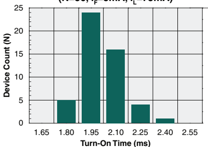
Typical Turn-On Time (N=50, I_F=5\text{mA} , I_L=75\text{mA} )
