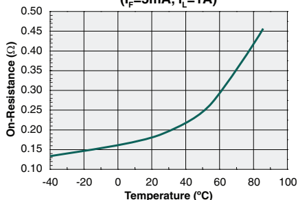
Typical On-Resistance vs. Temperature AC/DC Configuration ( I_F=5mA , I_L=1A )
