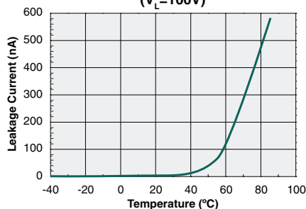
Leakage Current vs. Temperature Measured Across Pins 4&6 ( V_L=100V )
