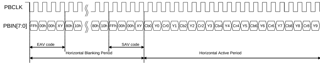
FIGURE 8 TIMING DIAGRAM OF ITU-R BT.656 FORMAT FOR DIGITAL VIDEO INPUT
