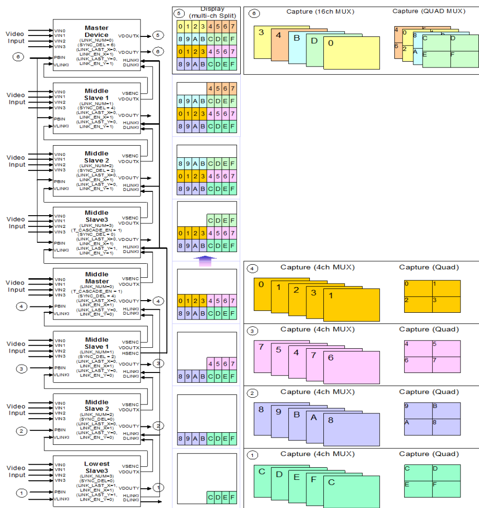
FIGURE 51 INFINITE CASCADE MODE FOR DISPLAY PATH
