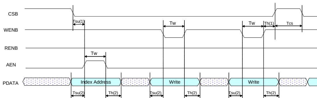
FIGURE 83 WRITE TIMING OF PARALLEL INTERFACE WITH AUTO INDEX INCREMENT MODE
