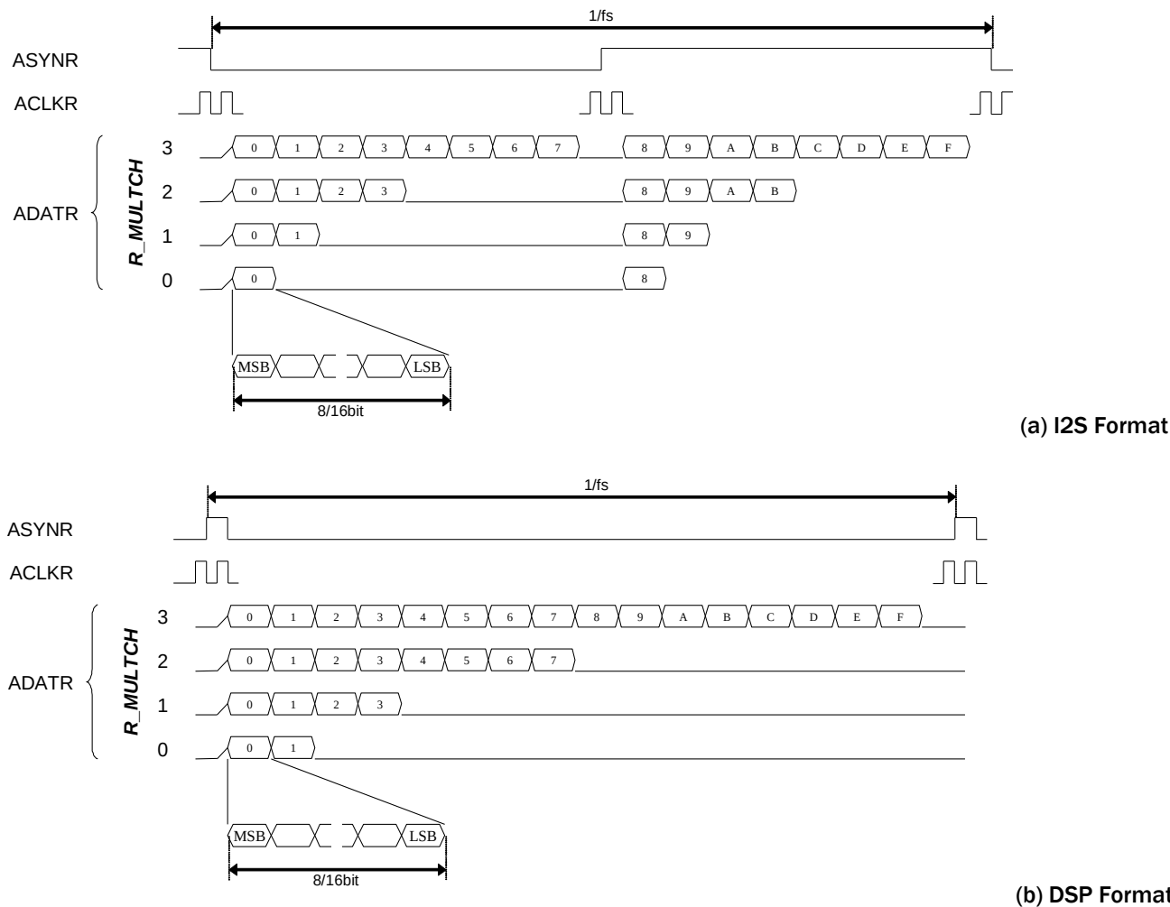
FIGURE 74 TIMING CHART OF MULTI-CHANNEL AUDIO RECORD
