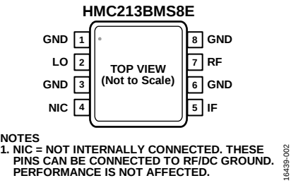
Figure 2. Pin Configuration
