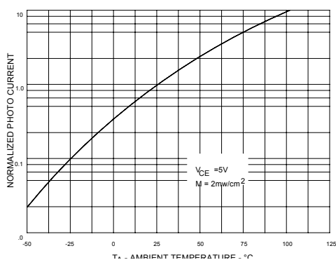
PHOTO CURRENT versus TEMPERATURE
