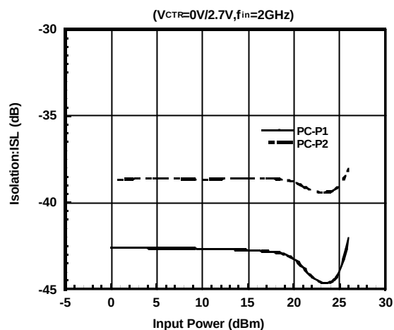
Isolation vs. Input Power
