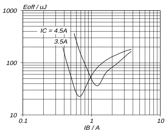
Fig.11. Typical turn-off losses. T_J = 85^\circ\text{C} E_{\text{off}} = f(I_B) ; parameter I_C ; f = 16\text{ kHz}
