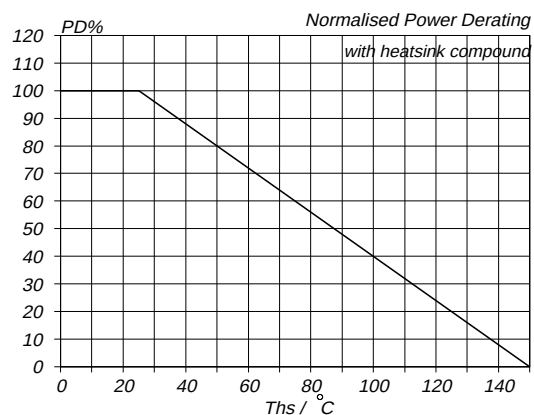
Fig.14. Normalised power dissipation.
