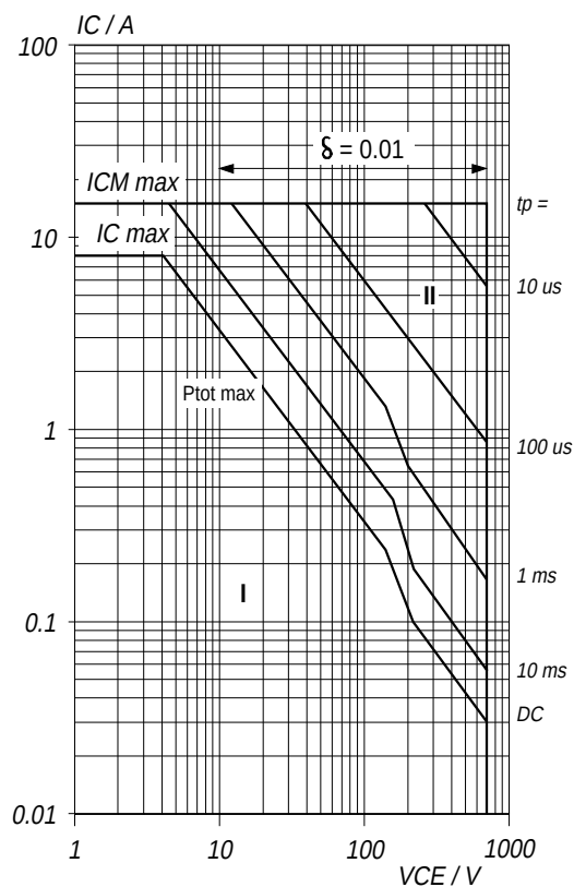
Fig.15. Forward bias safe operating area. T_{hs} = 25^{\circ}\text{C}
