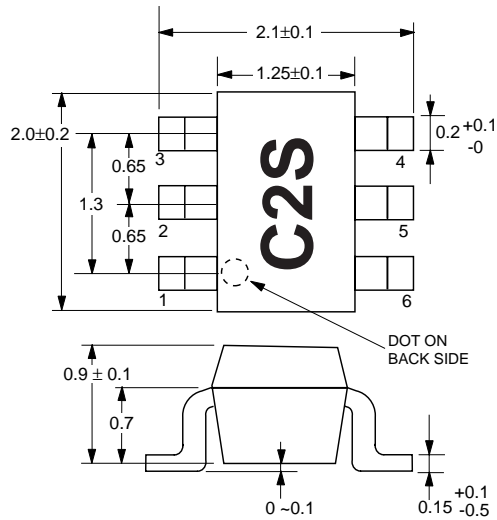
PACKAGE OUTLINE S06
