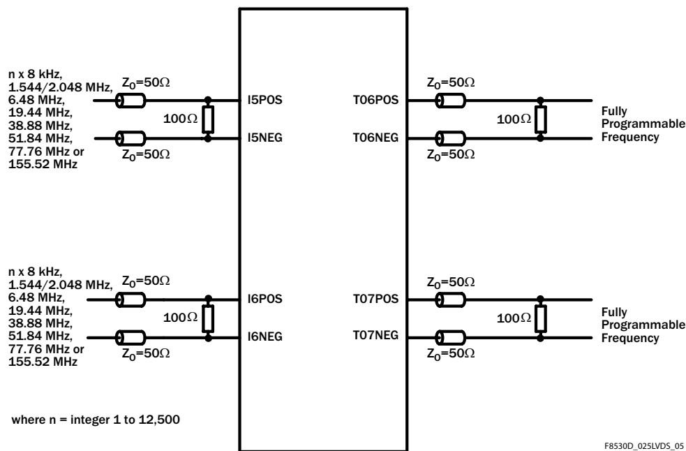
Figure 24 Recommended Line Termination for LVDS Input/Output Ports
