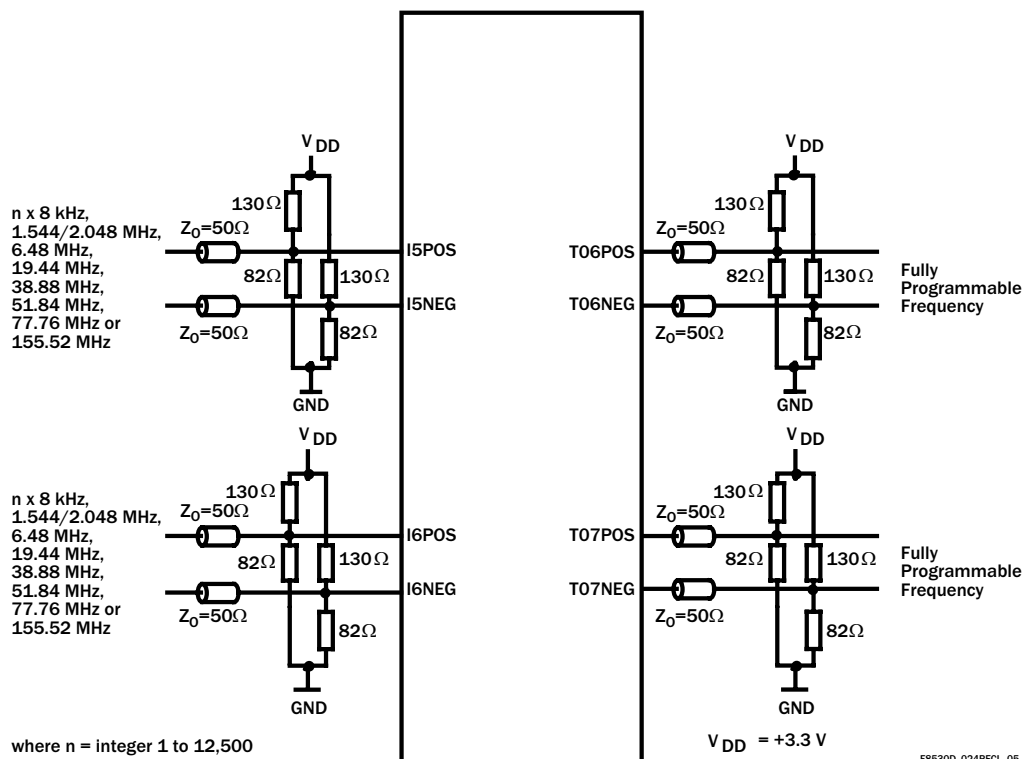
Figure 23 Recommended Line Termination for PECL Input/Output Ports
