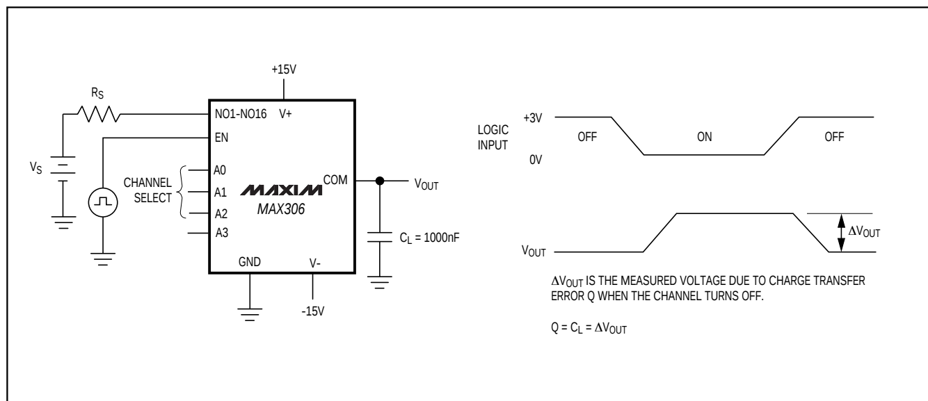
Figure 5. Charge Injection
