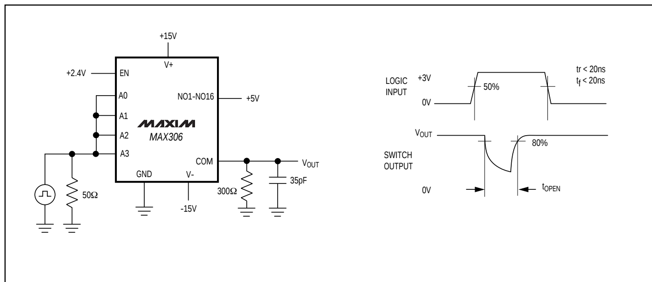
Figure 4. Break-Before-Make Interval
