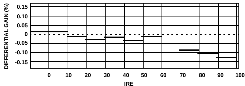
FIGURE 37. DIFFERENTIAL GAIN (%)
