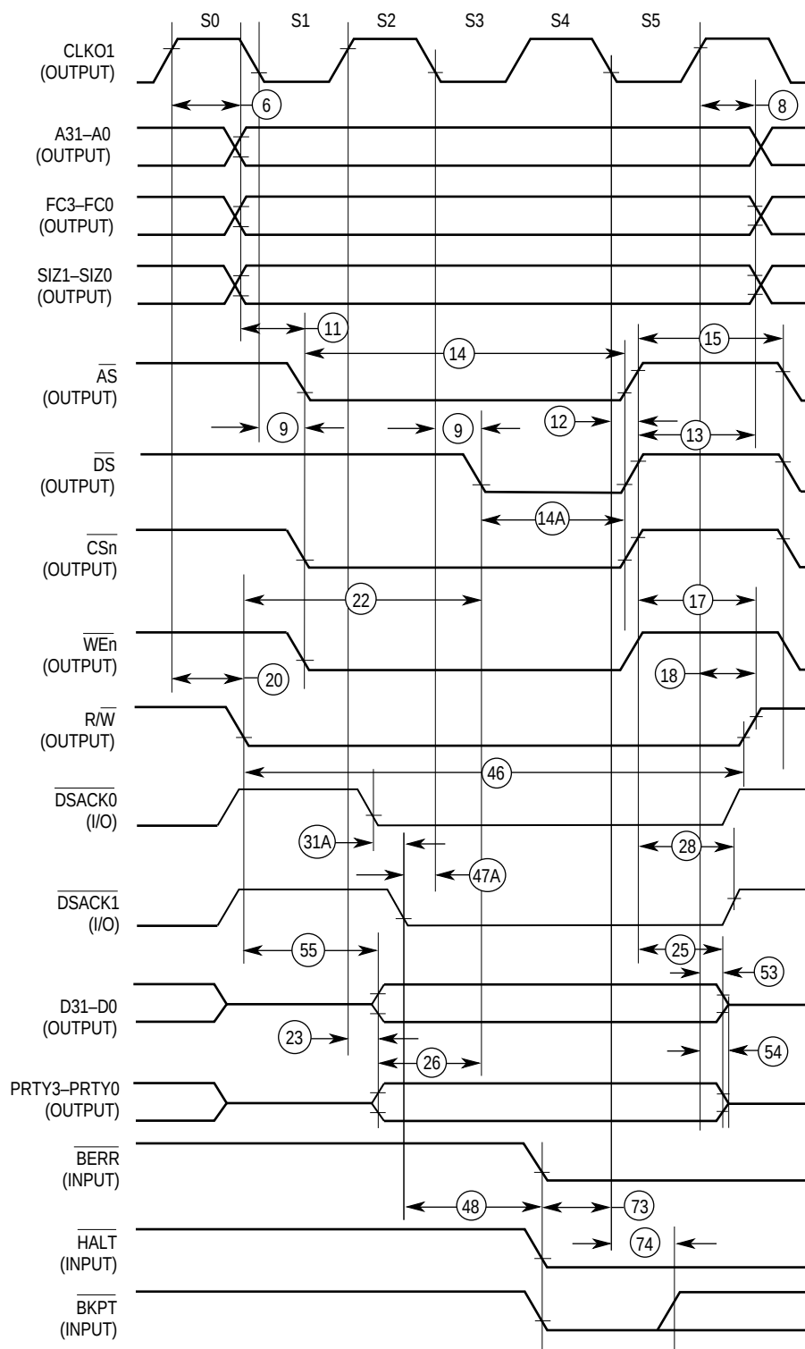
Figure 10-8. Write Cycle
