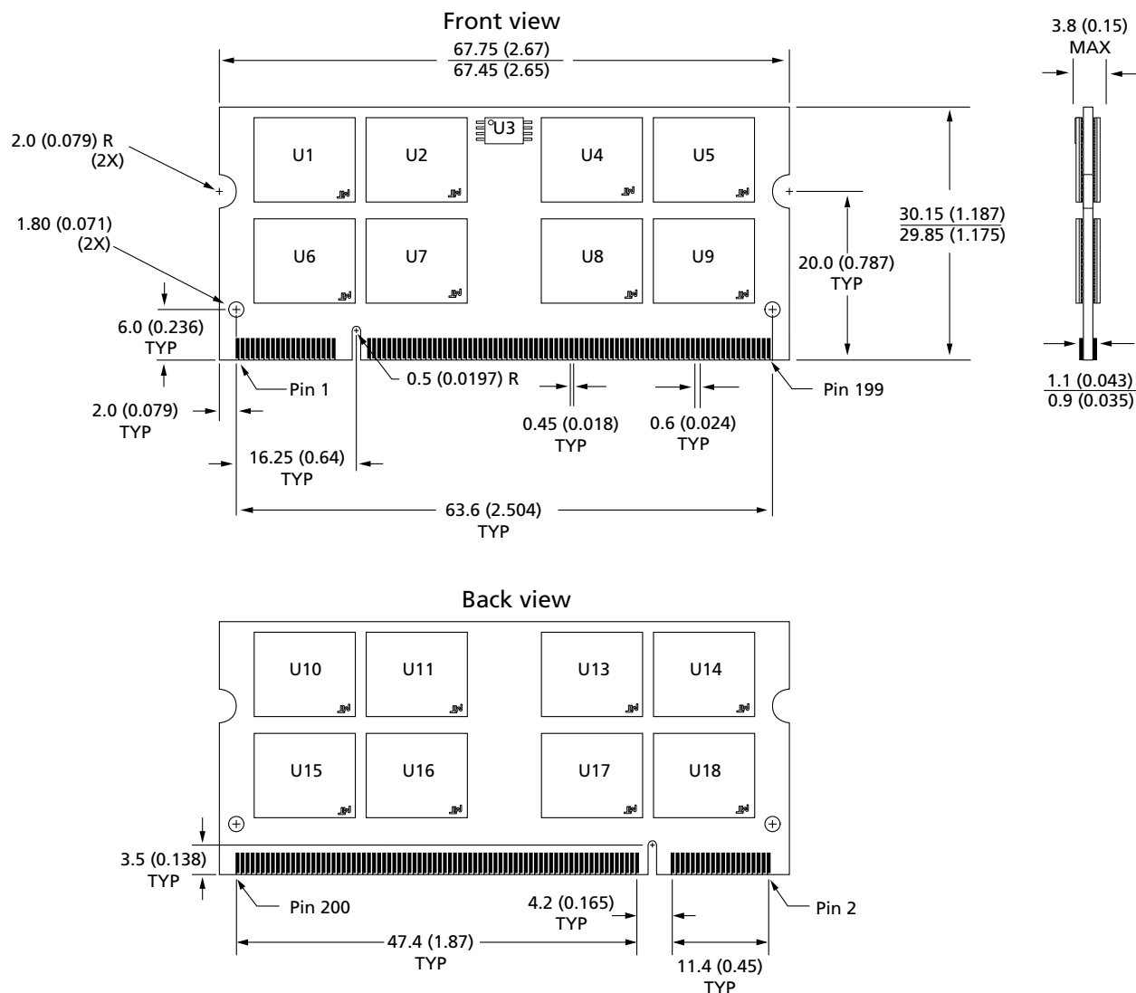
Figure 4: 200-Pin DDR2 SODIMM – 1GB, 2GB
