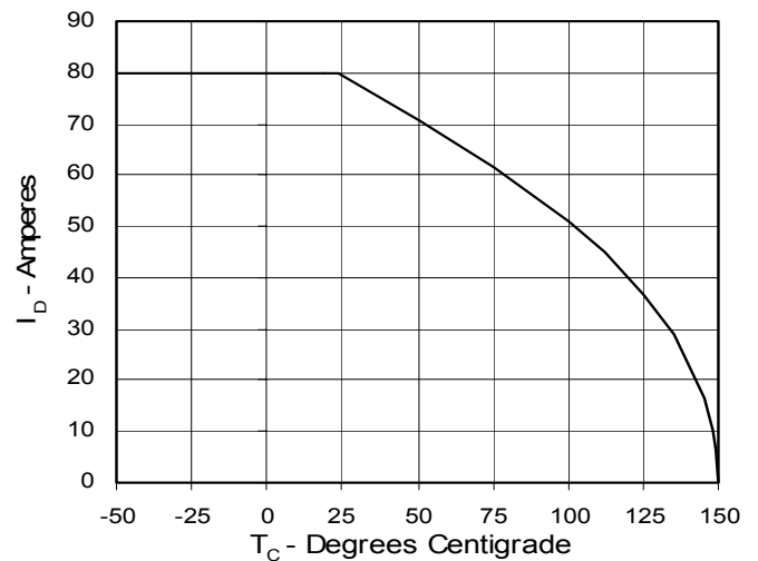
Fig. 6. Drain Current vs. Case Temperature
