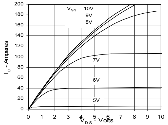
Fig. 2. Extended Output Characteristics @ 25 deg. C
