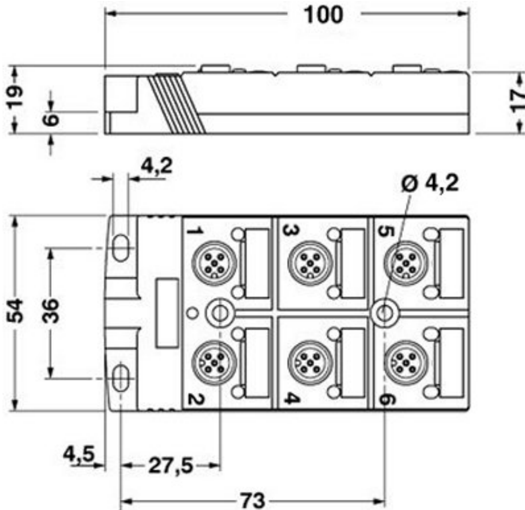
Dimensioned drawing
