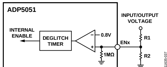
Figure 38. Precision Enable Diagram for a Single Channel
