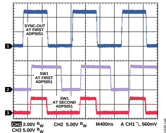
Figure 43. Waveforms of Two ADP5051 Devices Operating in Synchronization Mode
