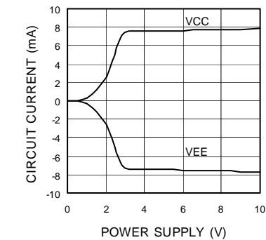
Fig.7 Circuit Current - Power Supply
