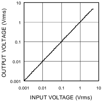
Fig.9 Output Voltage - Input Voltage
