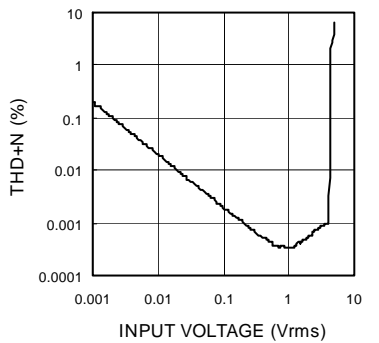
Fig.10 THD+N -Input Voltage
