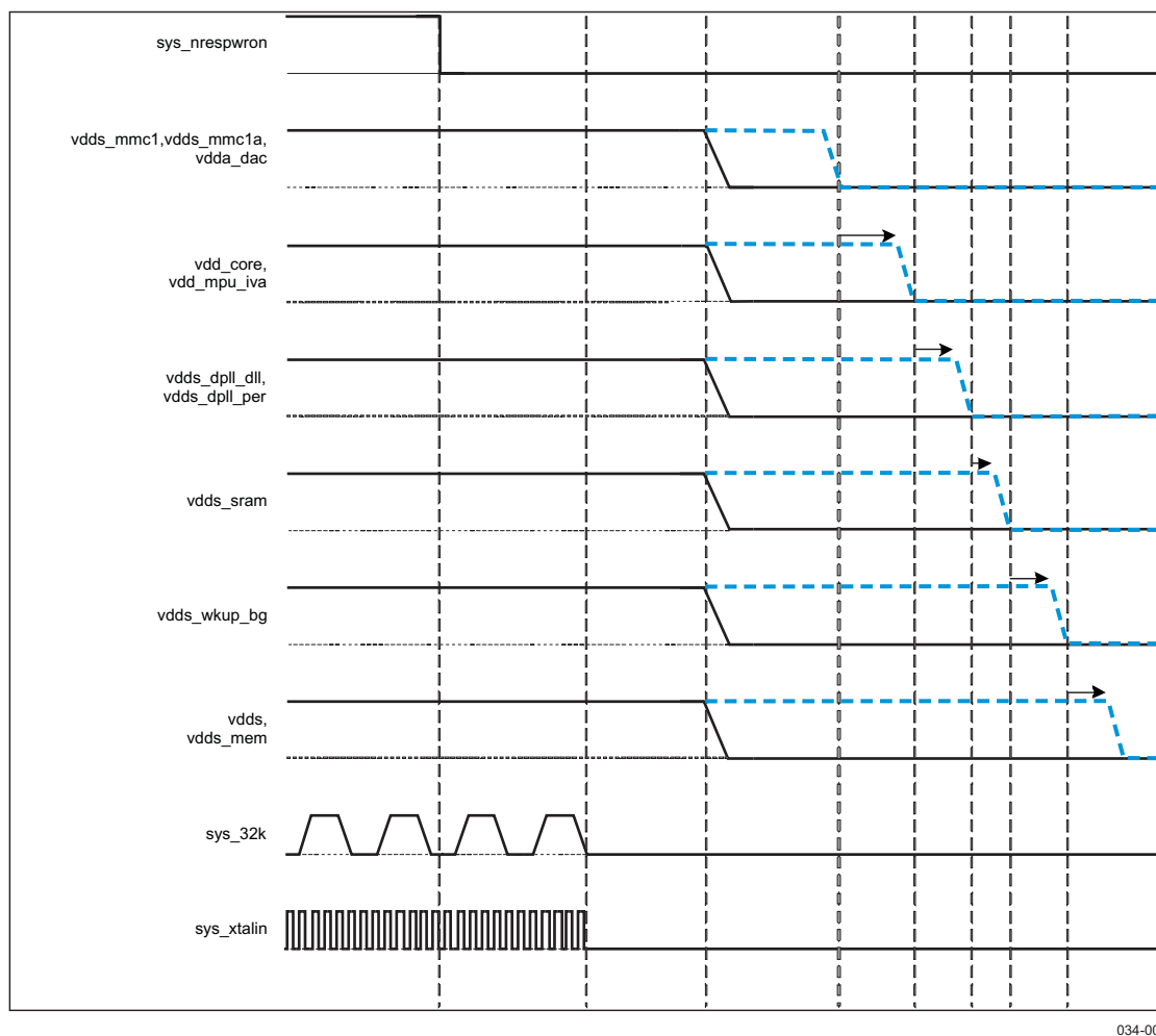
Figure 3-4. Power-down Sequence
