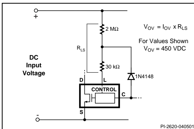
Figure 19. Line-Sensing for Overvoltage Only (Under-Voltage Disabled). Maximum Duty Cycle will be reduced at Low Line.
