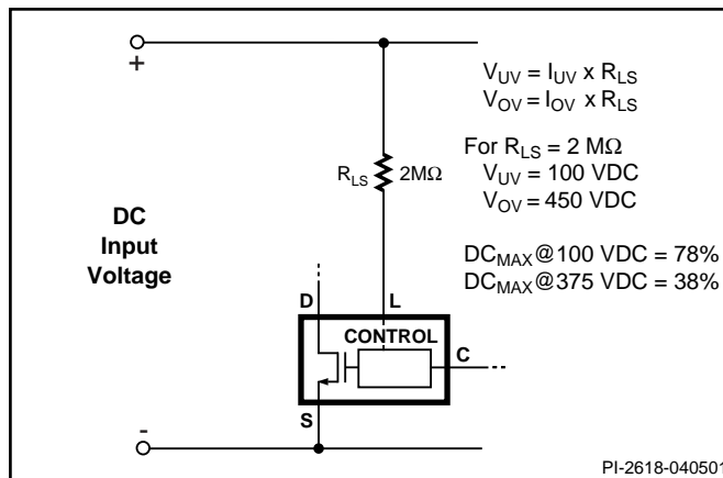
Figure 17. Line-Sensing for Under-Voltage, Overvoltage and Line Feed Forward.
