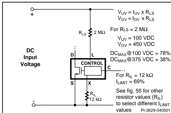
Figure 4. Y/R/F Package Line Sense and Externally Set Current Limit.
