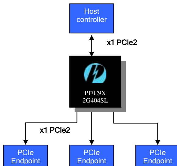
PI7C9X2G404SL – Application Example
