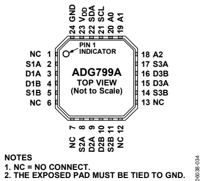
Figure 3. ADG799A Pin Configuration
