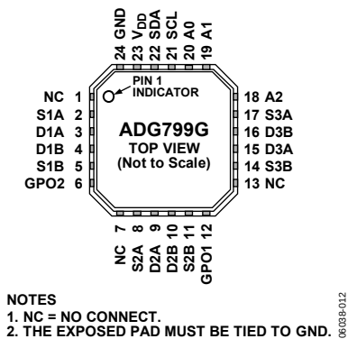
Figure 4. ADG799G Pin Configuration
