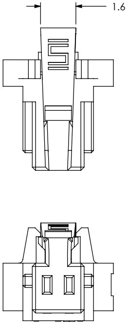
FIG 2 ISS1-02-L SHOWN (DIFFERENT AS SHOWN, OTHERWISE SAME AS FIG 1) (FOR POSITIONS -02 THRU -04)
