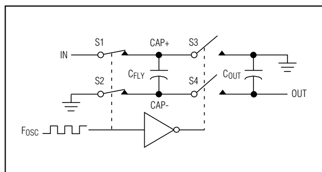
Figure 2. Charging C_{\text{FLY}}
