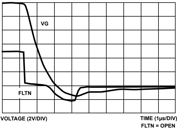
FIGURE 20. FLTN TO 35VG DELAY
