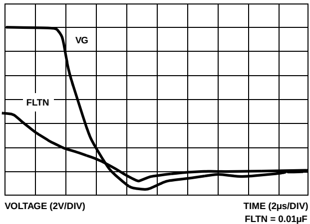
FIGURE 22. FLTN TO 35VG DELAY
