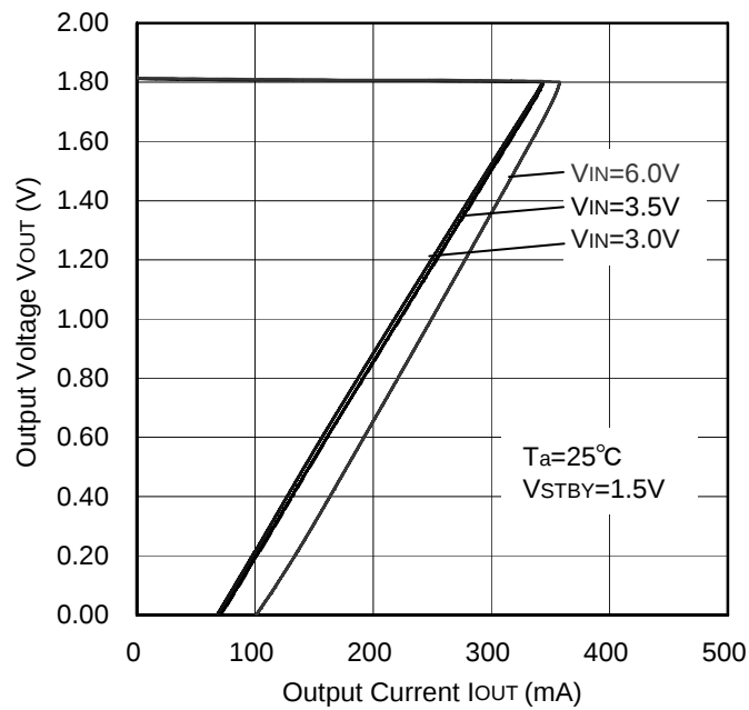
Figure 30. OCP Threshold
