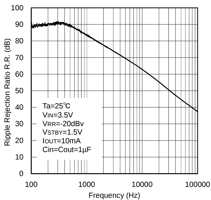
Figure 14. Ripple Rejection Ratio vs. Frequency
