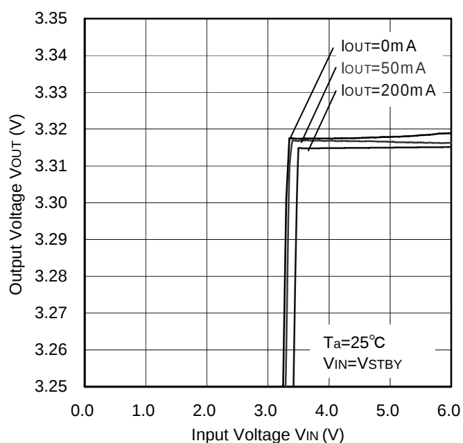
Figure 71. Line Regulation
