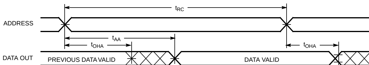
Figure 5. Read Cycle No. 2 (Either Port \overline{\text{CE}}/\overline{\text{OE}} Access) [15, 18, 19]
