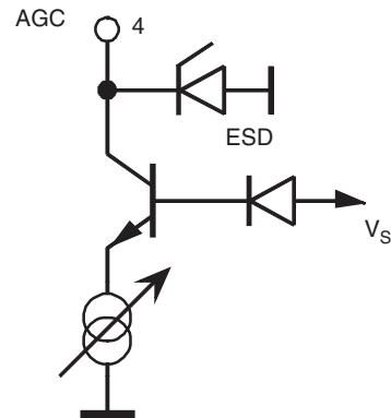
Figure 3-3. Internal Circuit at Pin AGC
