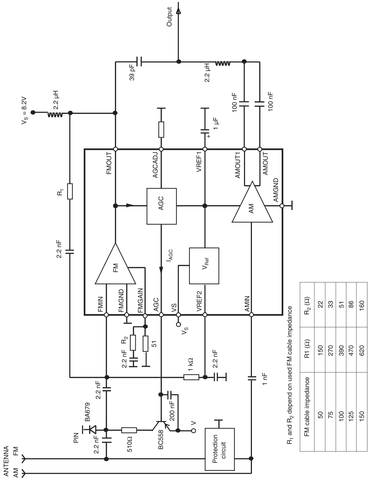
Figure 7-5. Application Circuit
