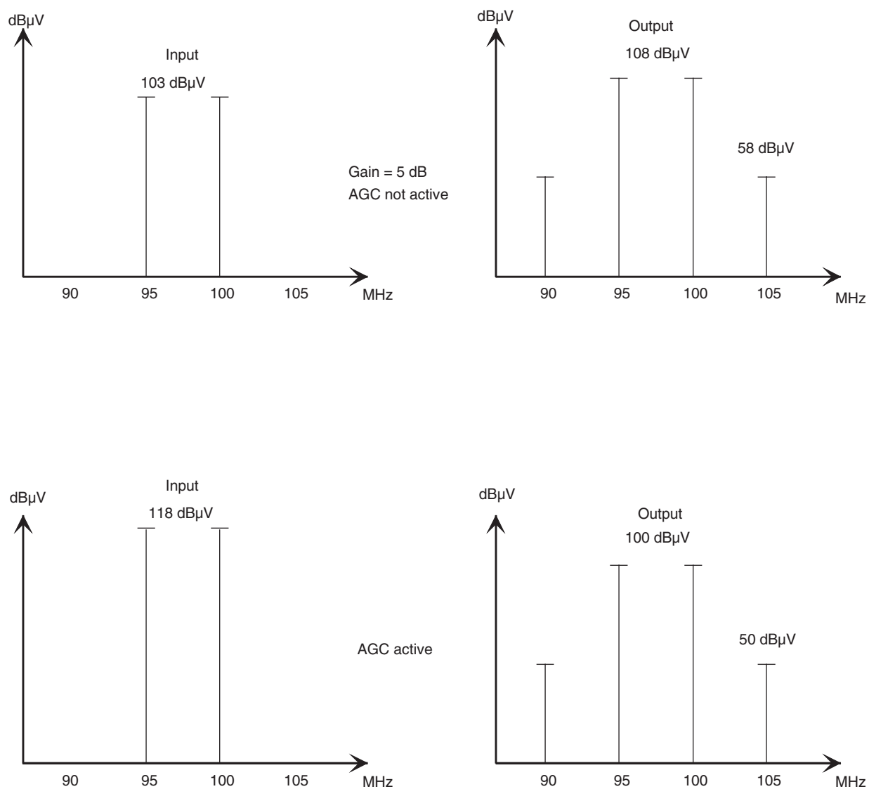
Figure 7-2. FM Intermodulation Distortion
