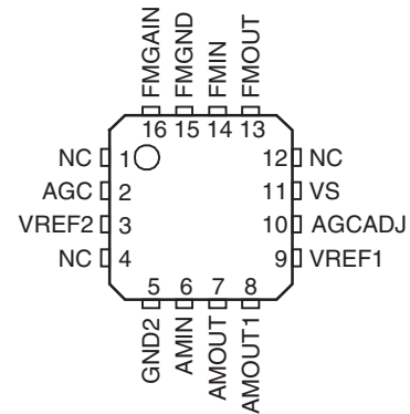
Figure 2-2. Pinning QFN16 4 × 4
