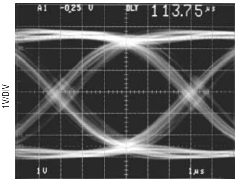
Eye Diagram
