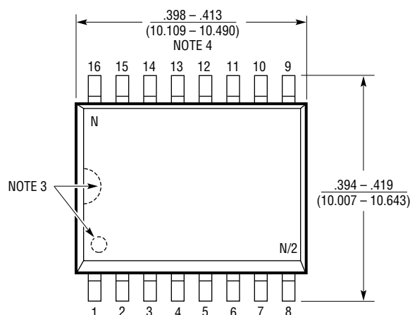
SW Package 16-Lead Plastic Small Outline (Wide .300 Inch) (Reference LTC DWG # 05-08-1620)
