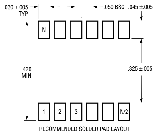
SW Package 16-Lead Plastic Small Outline (Wide .300 Inch) (Reference LTC DWG # 05-08-1620)
