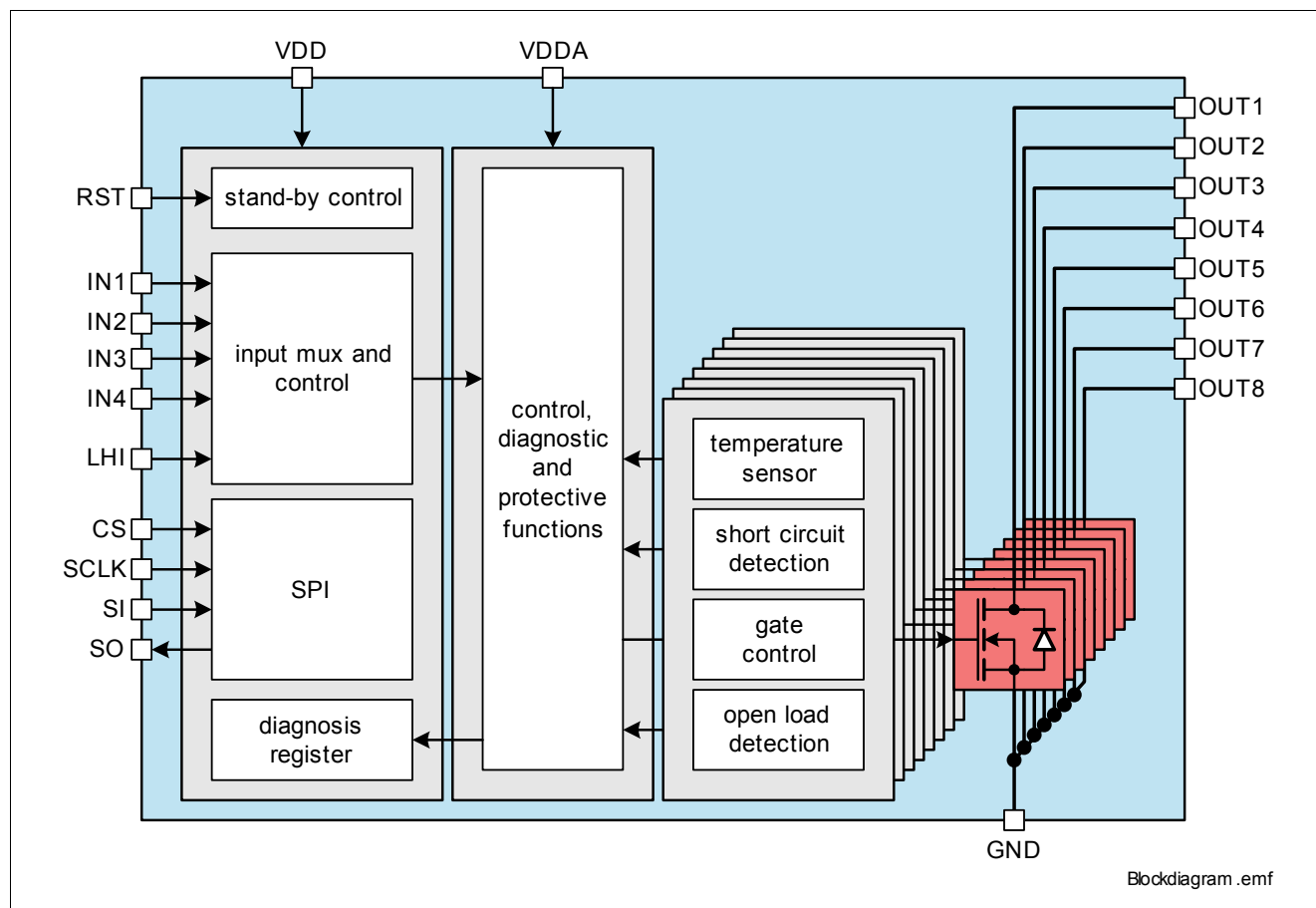
Figure 1 Block Diagram for the SPIDER - TLE 7240SL
