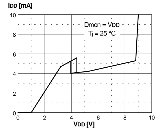
Figure 2. IC Supply current vs. supply voltage
