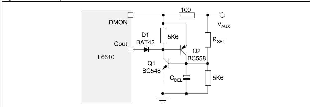
Figure 27. Auxiliary OVP without Crowbar
