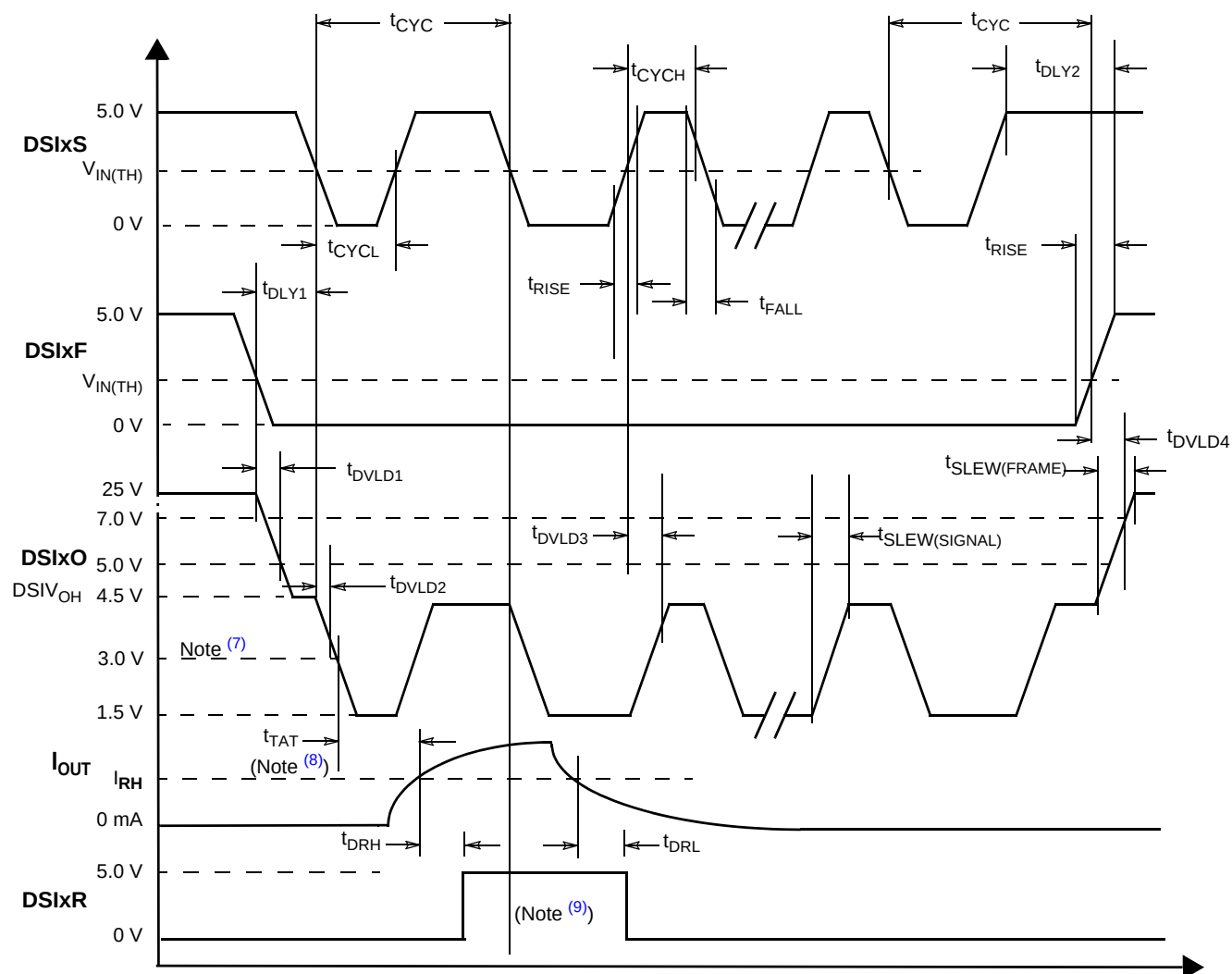
Figure 4. Timing Characteristics
