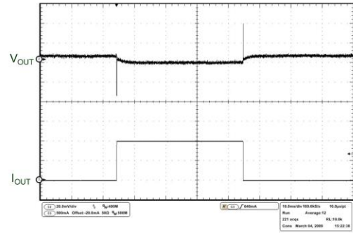
Figure 25: Load Transient ( V_{OUT} = 2.5\text{ V} , I_{OUT} = \text{from } 10\text{ mA to } 1\text{ A} )
