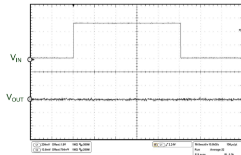
Figure 27: Line transient
