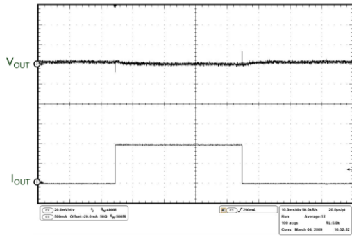
Figure 24: Load Transient ( V_{OUT} = 0.8\text{ V} , I_{OUT} = \text{from } 100\text{ mA to } 1\text{ A} )
