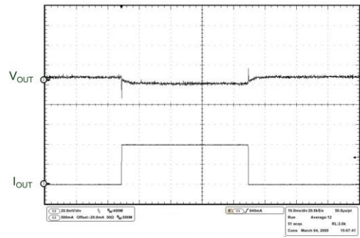
Figure 26: Load Transient ( V_{OUT} = 2.5\text{ V} , I_{OUT} = \text{from } 100\text{ mA to } 1\text{ A} )
