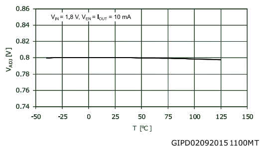
Figure 4: V_{ADJ} accuracy
