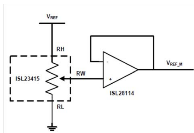
FIGURE 2. V_{\text{REF}} ADJUSTMENT
