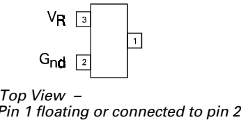
SOT23 Package Suffix – F
