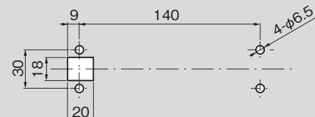
[A-869-2] パネル穴明け寸法 Panel drilling dimensions
