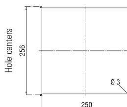
Enclosure cut-out
