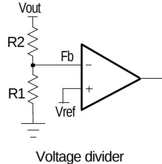
Figure 8 - Voltage divider
