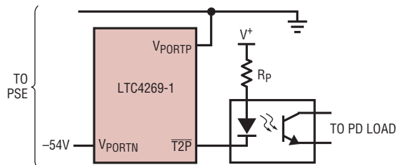
OPTION 1: SERIES CONFIGURATION FOR ACTIVE LOW/LOW IMPEDANCE OUTPUT
