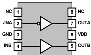
ISL89162FR, ISL89162FB (8 LD TDFN, EPSONIC) TOP VIEW
