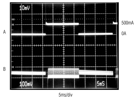
LOAD-TRANSIENT RESPONSE
