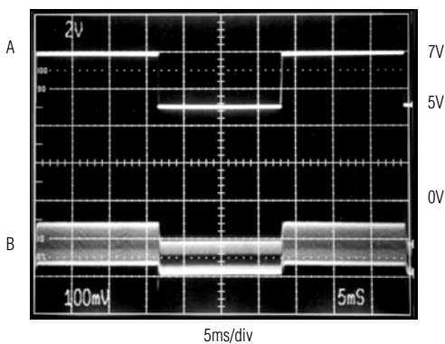
LINE-TRANSIENT RESPONSE
