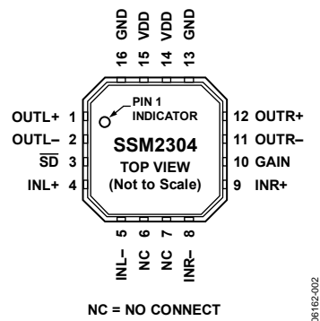
Figure 2. SSM2304 LFCSP Pin Configuration
