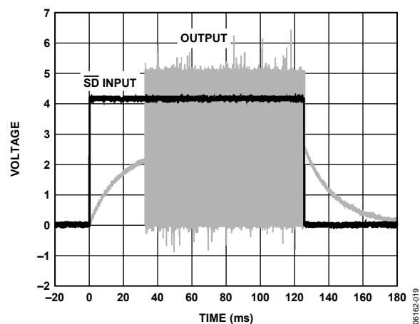
Figure 24. Turn-Off Response
