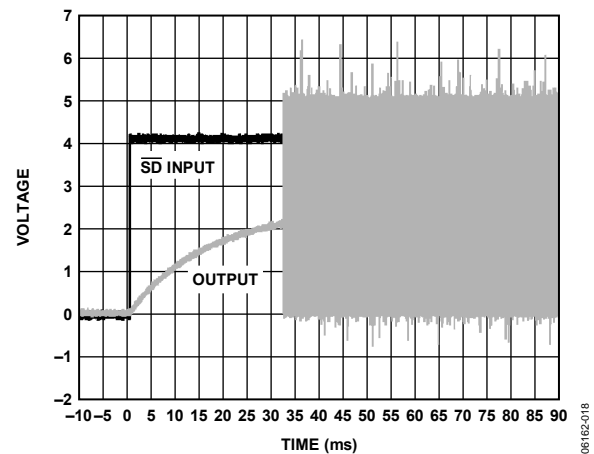
Figure 23. Turn-On Response
