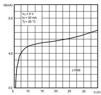
Figure 36. Quiescent current vs. input voltage
