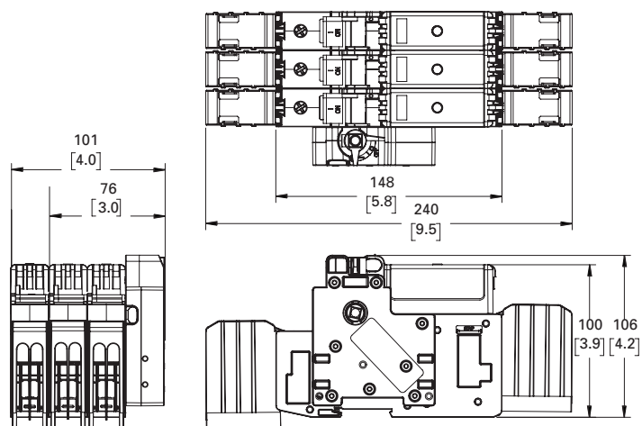
100 amp switches
