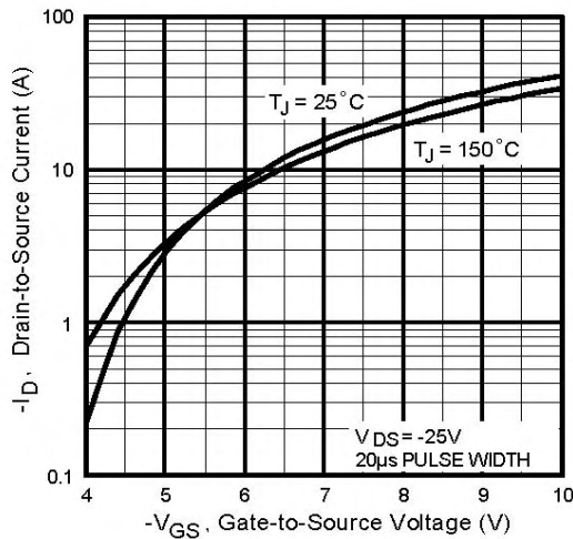
Fig 3. Typical Transfer Characteristics www.irf.com
