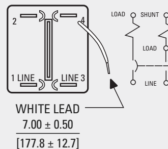
Two Pole ( 1 pole shunt)
