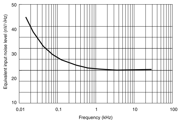
Figure 11. Equivalent input noise voltage vs. frequency
