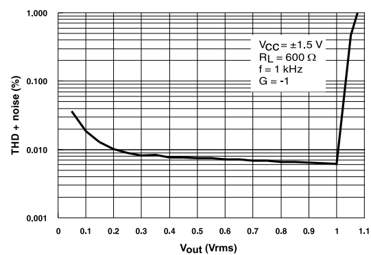
Figure 8. THD + noise vs. V_{out} , R_L = 600\ \Omega
