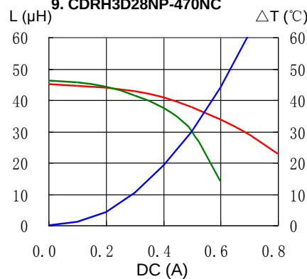
9. CDRH3D28NP-470NC
