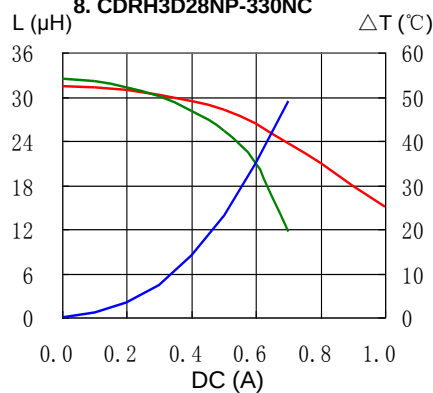
8. CDRH3D28NP-330NC
