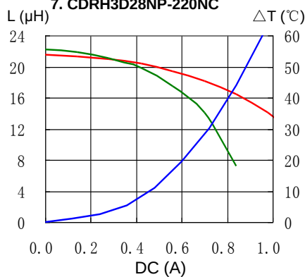
7. CDRH3D28NP-220NC
