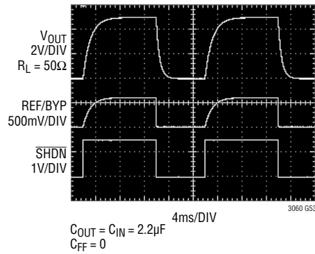
SHDN Transient Response C_{\text{REF/BYP}} = 10\text{nF}
