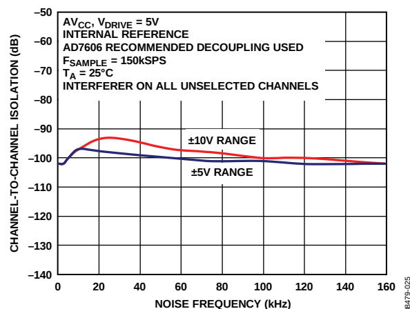
Figure 28. Channel-to-Channel Isolation
