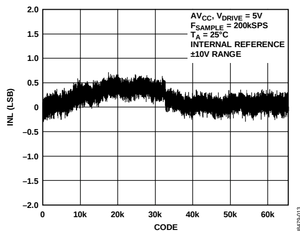
Figure 14. AD7606 Typical INL, ±10 V Range
