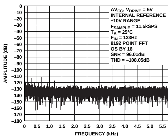
Figure 13. FFT Plot Oversampling By 16, ±10 V Range
