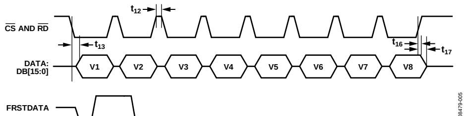
Figure 5. \overline{\text{CS}} and \overline{\text{RD}} , Linked Parallel Mode
