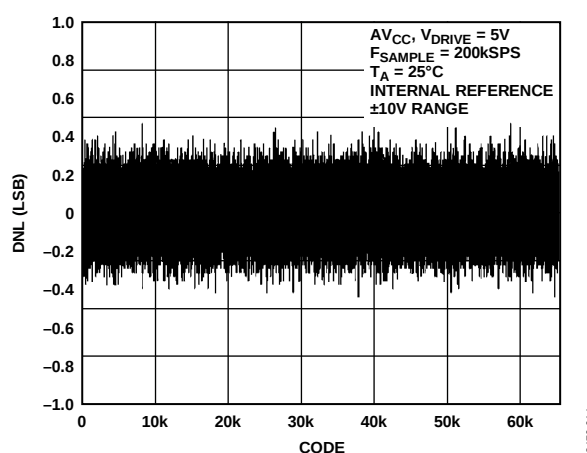
Figure 15. AD7606 Typical DNL, ±10 V Range
