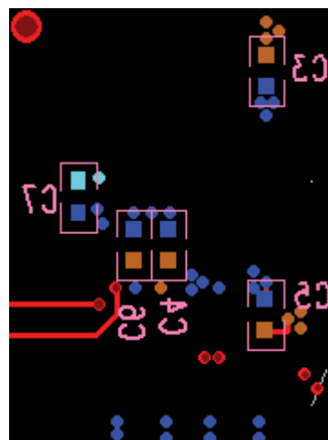
Figure 63. Bottom Layer Decoupling
