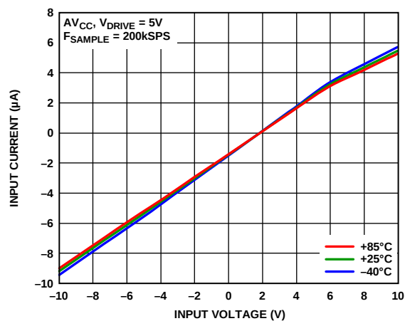
Figure 31. Analog Input Current vs. Temperature for Various Supply Voltages
