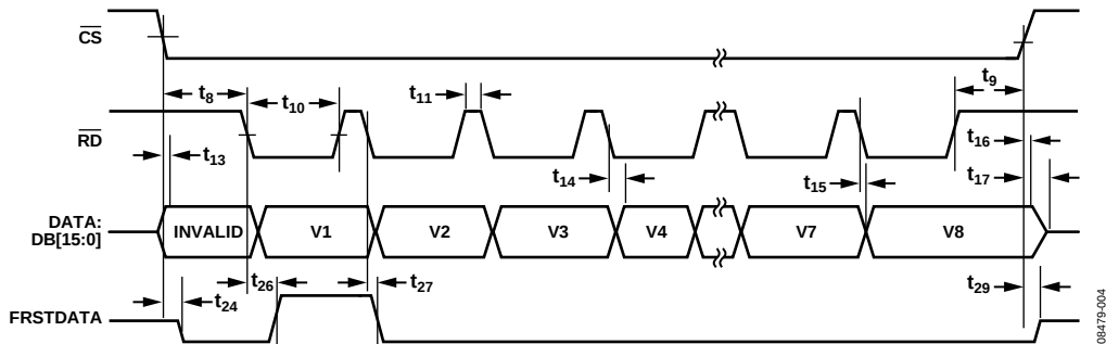
Figure 4. Parallel Mode, Separate \overline{\text{CS}} and \overline{\text{RD}} Pulses
